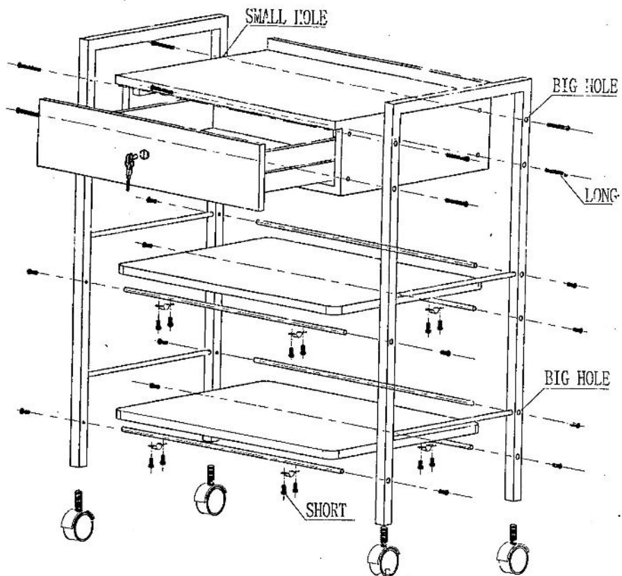
THE INSTALLATION DIAGRAM FOR 1019A TROLLEY
